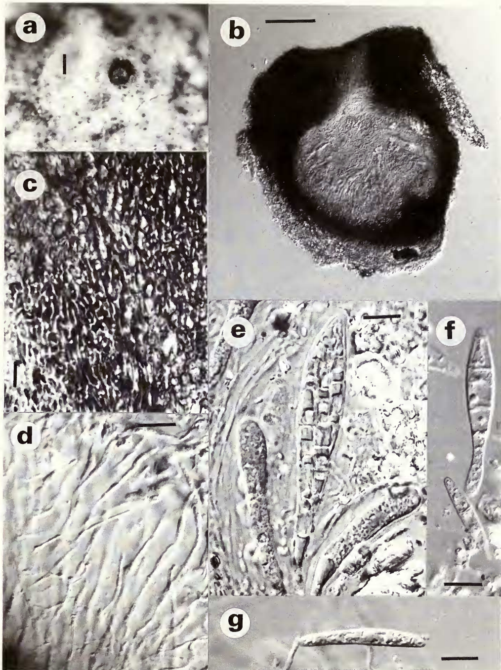
Fig. 73 Sagediopsis barbara (Th. Fr.) R. Sant & D. Triebel (WRSI-isolotype of Leptorhaphis steinii ) (a) Surface view of ascoma; scale = 500 \mu m; (b) Vertical section of ascoma; scale = 100 \mu m; (c) Detail of exciple: textura angularis and porrecta; (d) Periphyses in ostiolar channel; (e) Asci and ascospores; (f), (g) Ascospores; scale = 10 \mu m.
